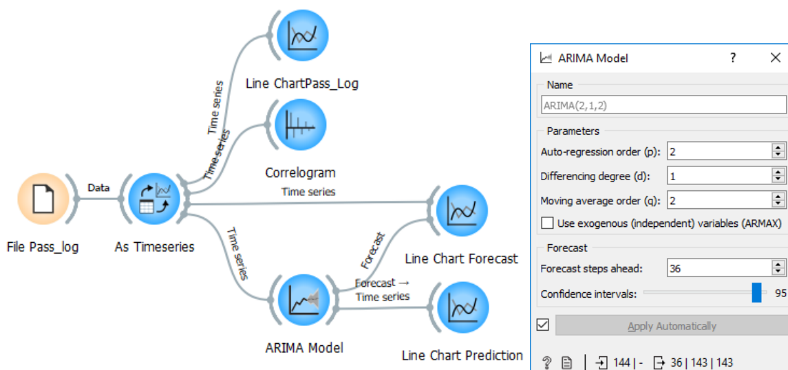
Obr. 193 Workflow s ARIMA modelem
