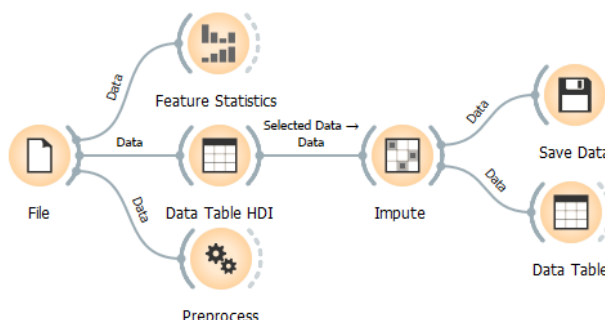
Obr. 23 Workflow s uzlem Impute a Preprocess pro imputaci hodnot
