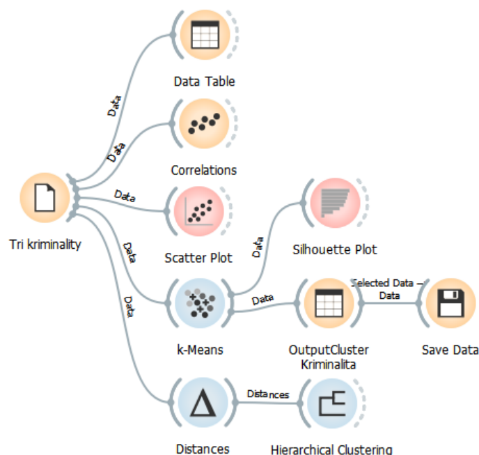
Obr. 71 Workflow s uzlem k-Means
