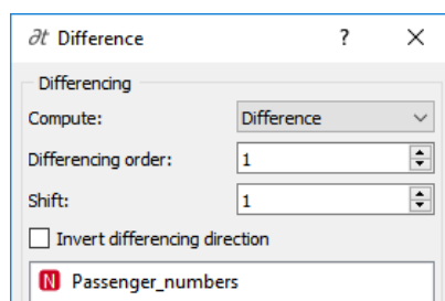
Obr. 181 Uzel Difference
