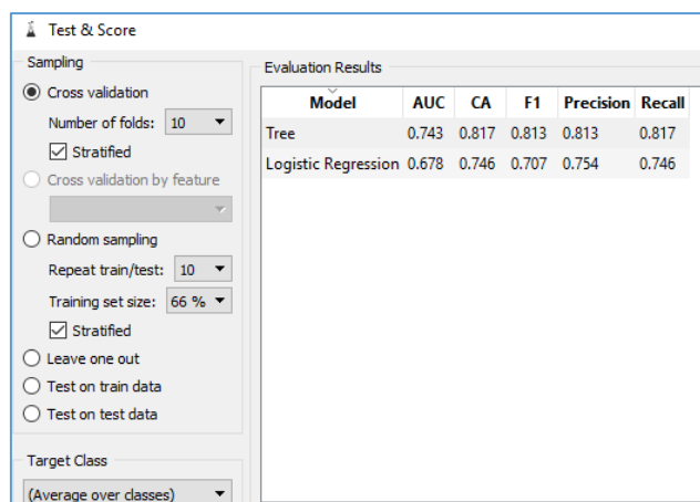
Obr. 106 Uzel Test &amp; Score
